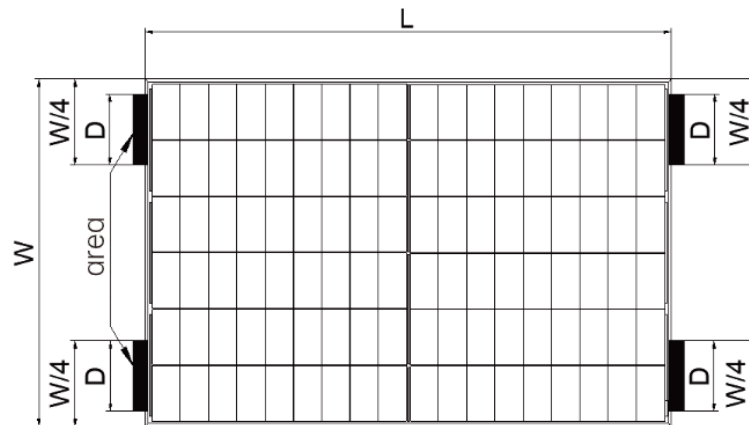
clamp mounting on short frame
